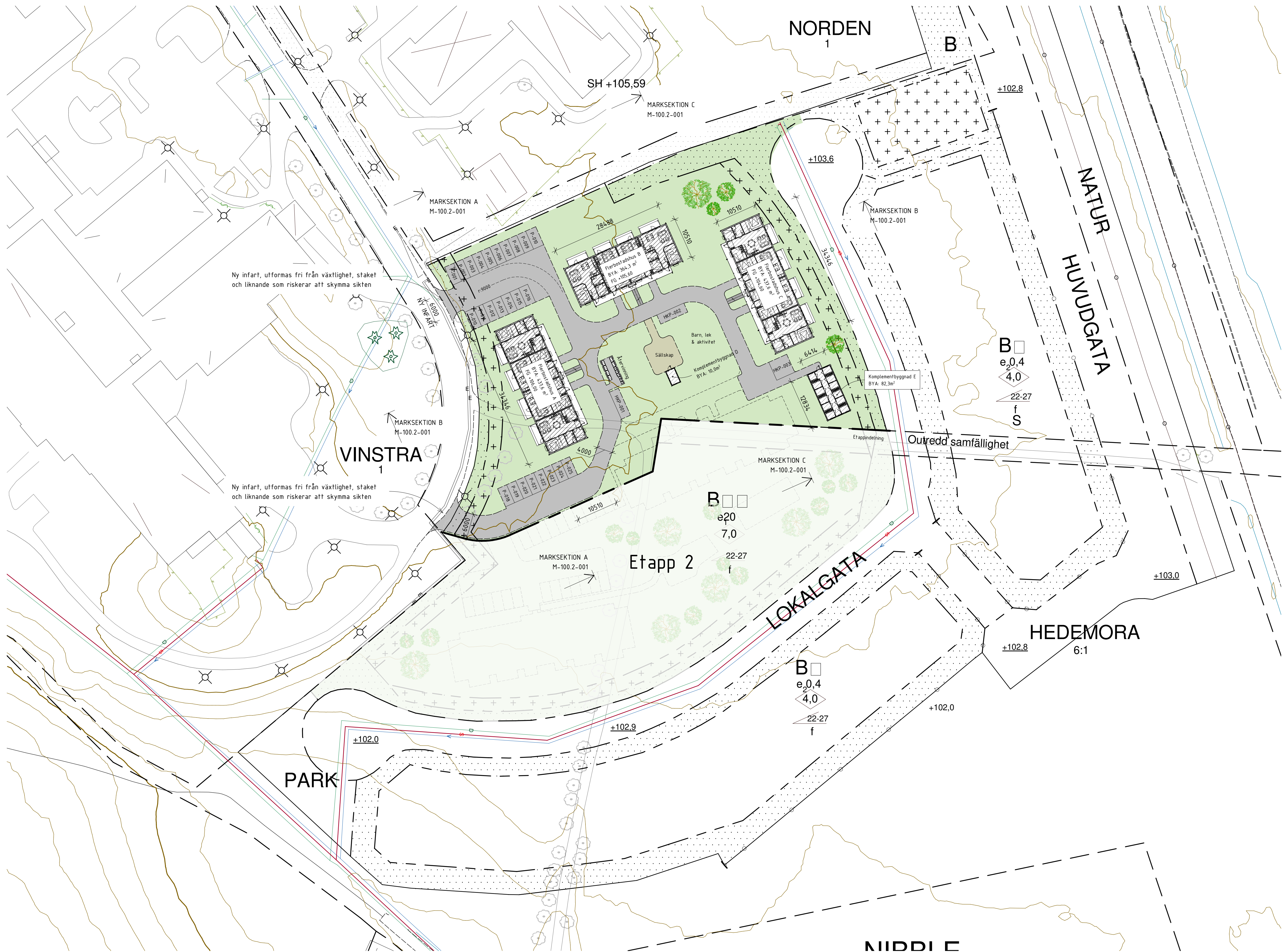
SITUATIONSPLAN
